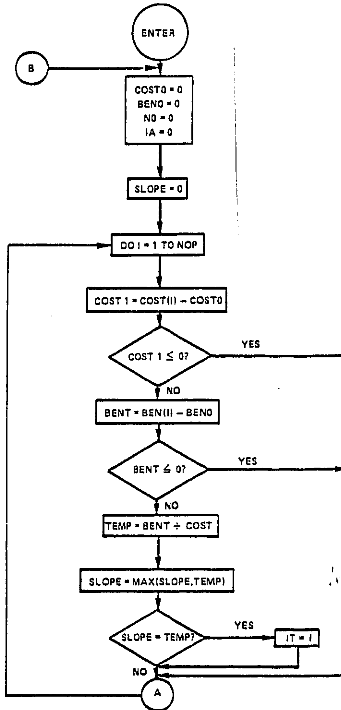
FIGURE 5-4. SUBROUTINE CONVEX FLOW CHART
