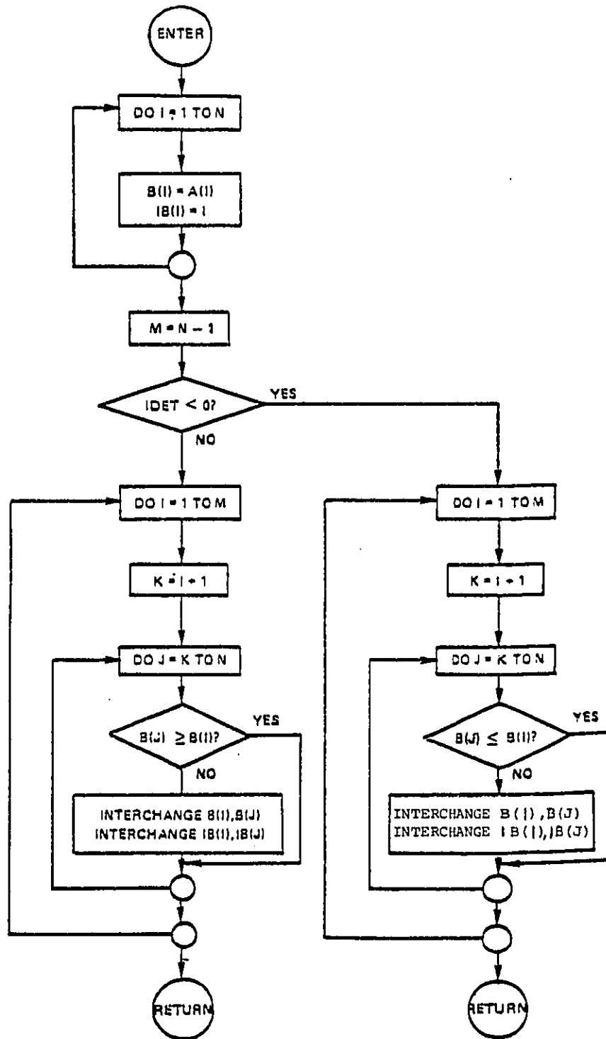
FIGURE 5-3. SUBROUTINE SORT FLOW CHART
