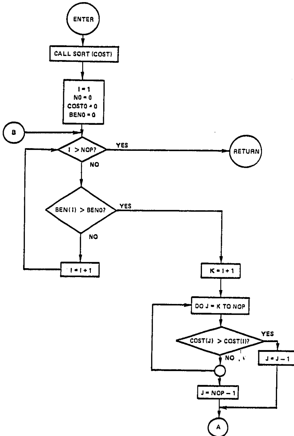
FIGURE 5-8. SUBROUTINE MONOTO FLOW CHART.
