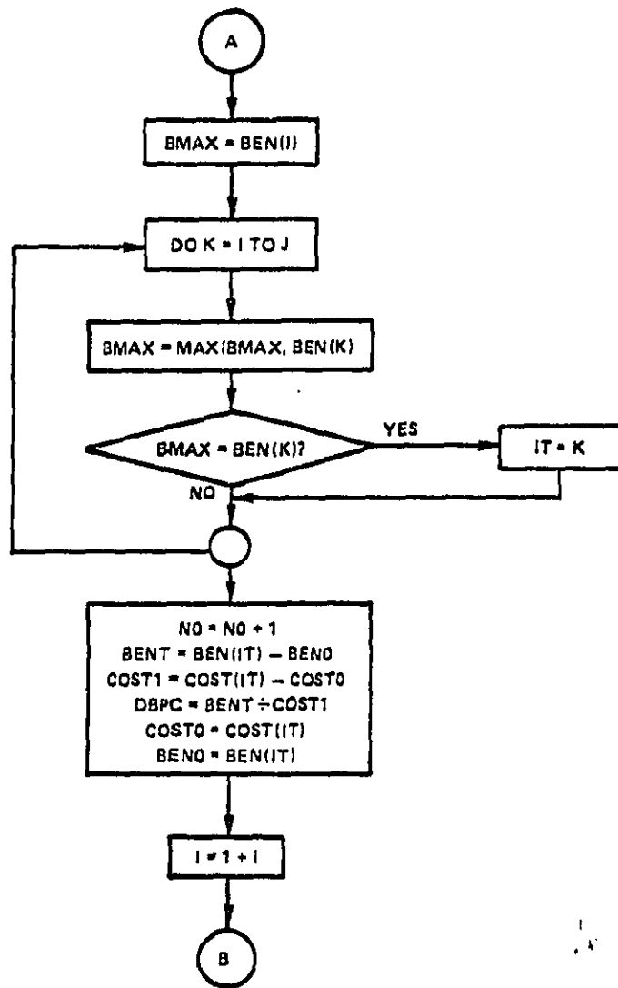
FIGURE 5-6. SUBROUTINE MONOTO FLOW CHART (CONTINUED)
